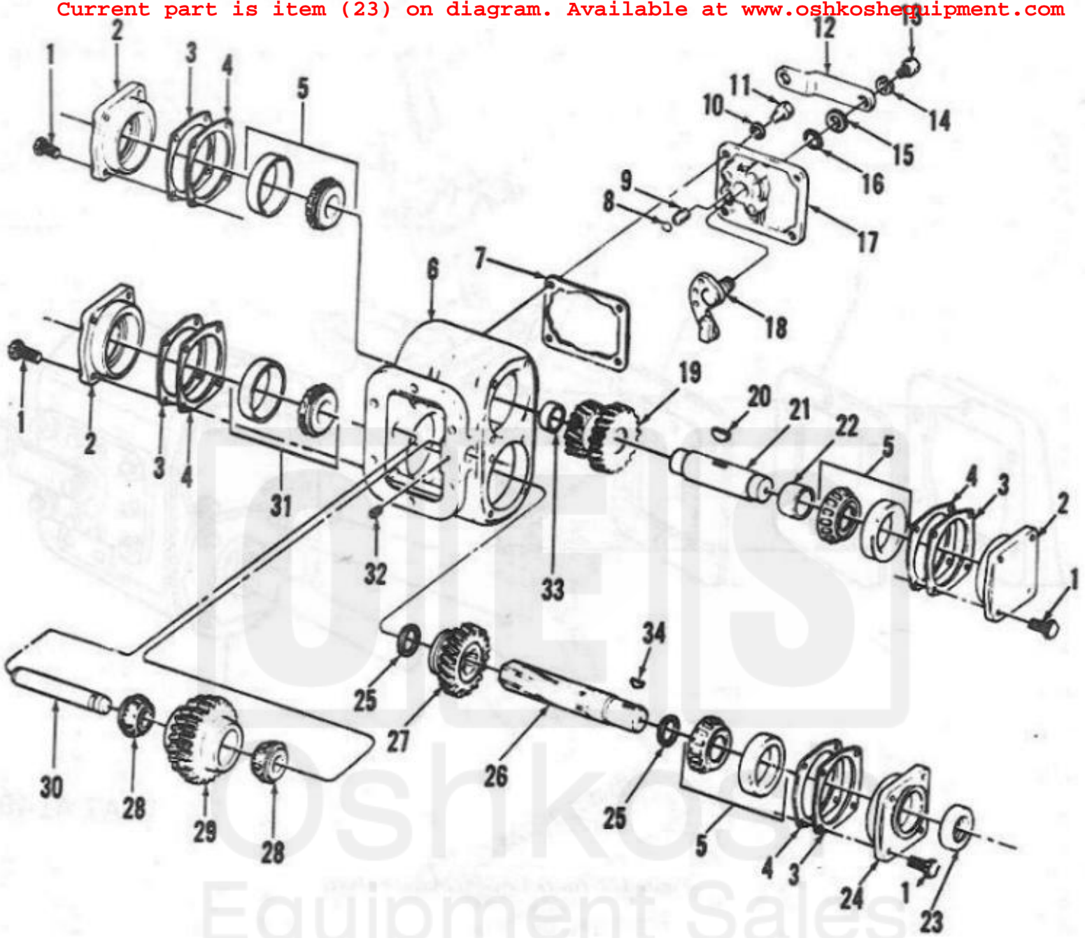
Figure 138: Power Take-Off Assembly Page 367
